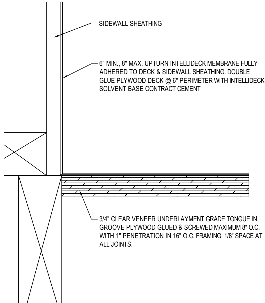
SECTION VIEW
